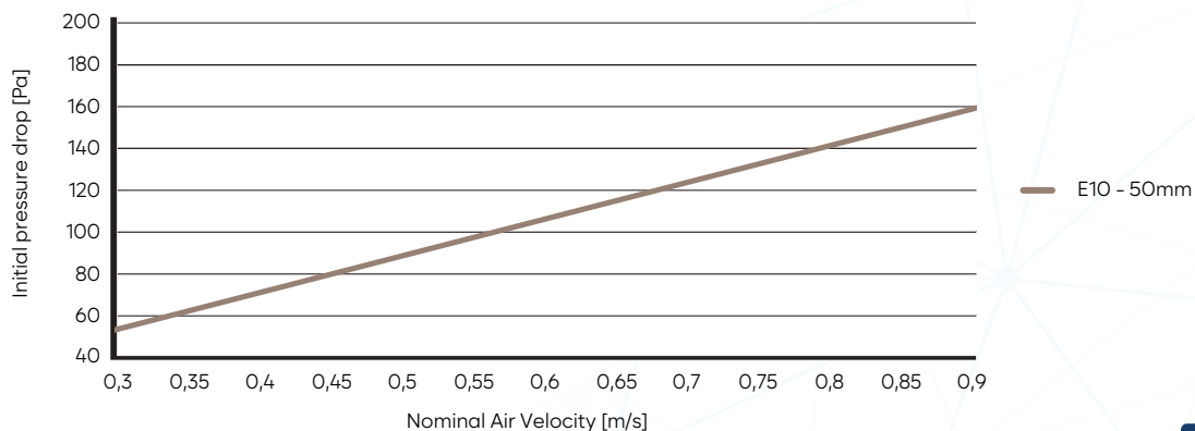
EPA Ceiling Filter - Pleat Code:1 (PH50)
