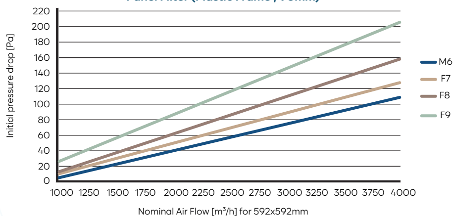
Panel Filter (Plastic Frame ; 96mm)
