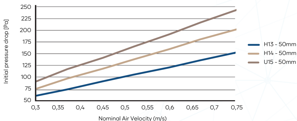
Terminal Hood Filter (Without Divider) - Pleat Code:1 (PH50)
