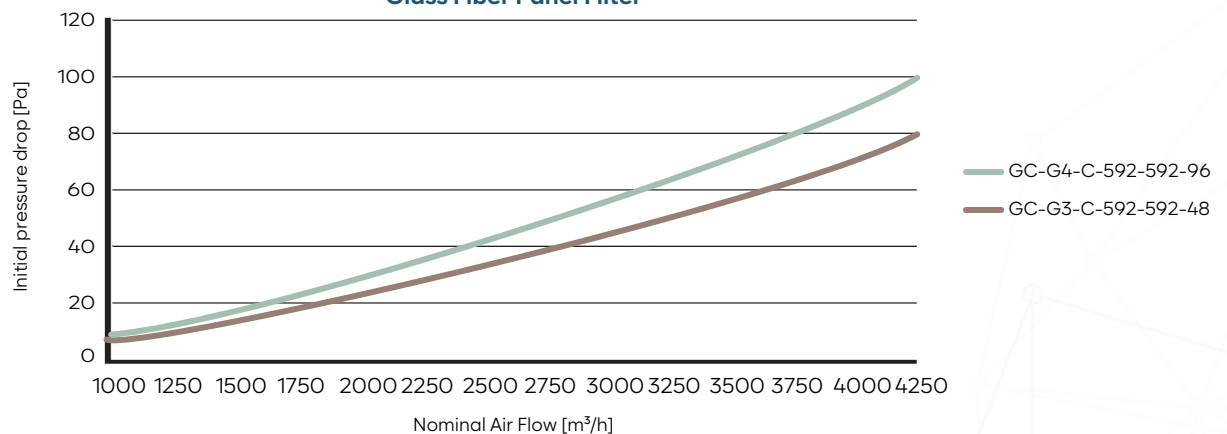
Glass Fiber Panel Filter
