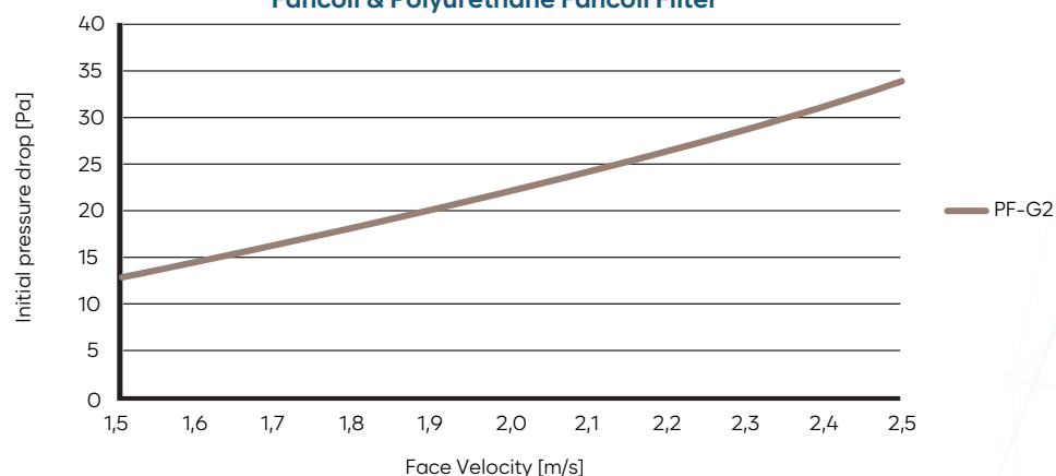
Fancoil & Polyurethane Fancoil Filter
