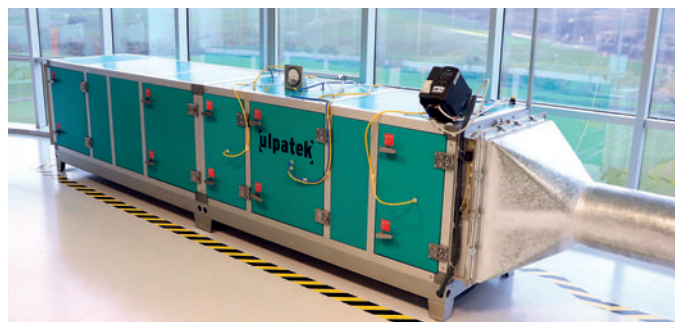
Performance Test System - PTS 5002
