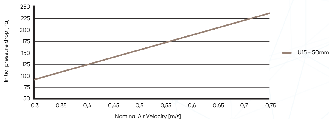
Knife Edge Ceiling Filter - Pleat Code:1 (PH50)
