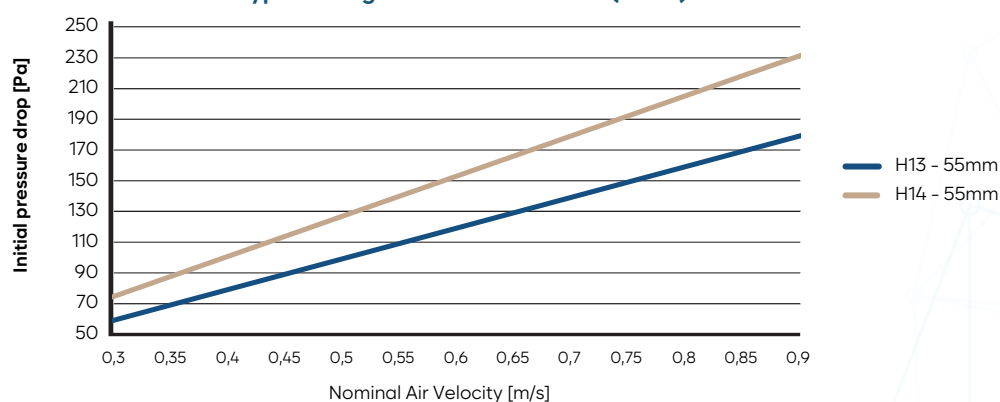
Gel Type Ceiling Filter - Pleat Code:J (PH55)
