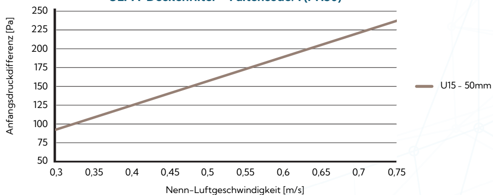
ULPA-Deckenfilter – Faltencode: 1 (PH50)
