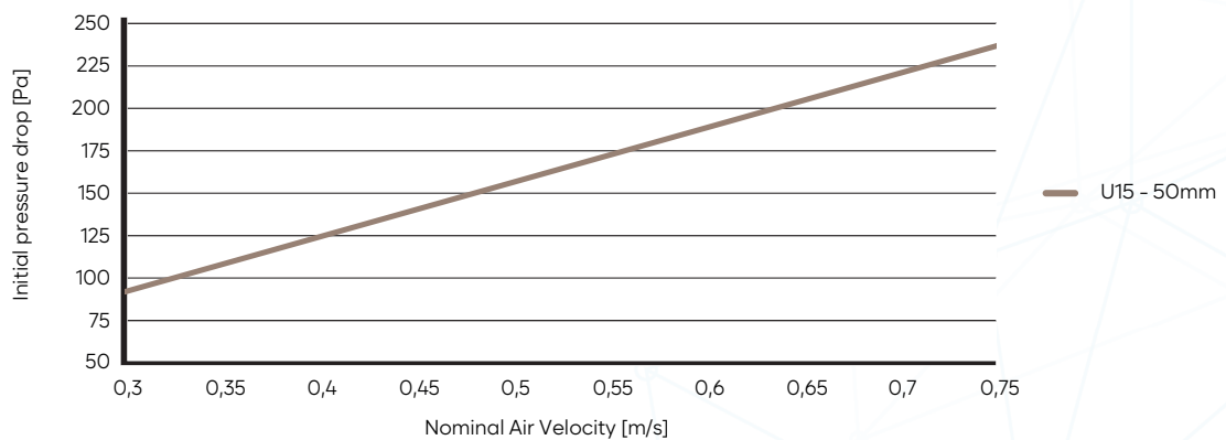
Knife Edge Ceiling Filter - Pleat Code:1 (PH50)
