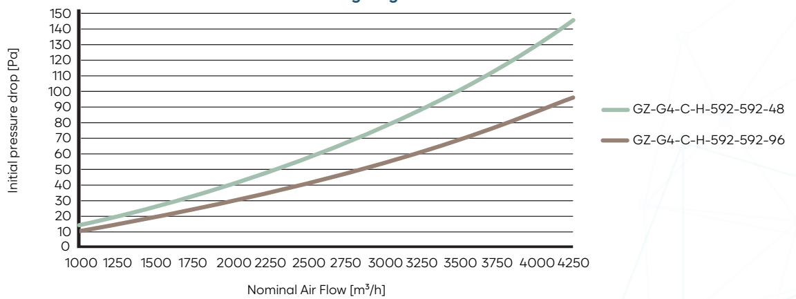
Cardboard Frame Zig-Zag Filter
